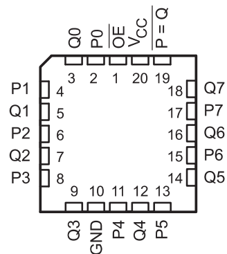
SN54F521 . . . FK PACKAGE (TOP VIEW)
