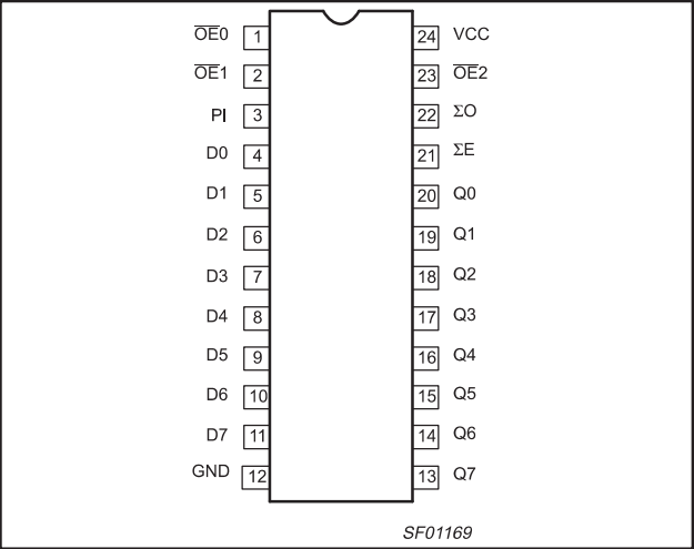
PIN CONFIGURATION – 74F656A
