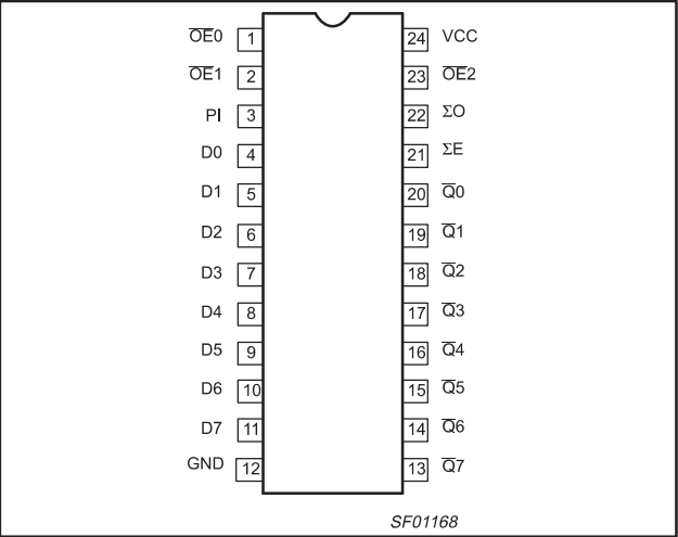
PIN CONFIGURATION – 74F655A
