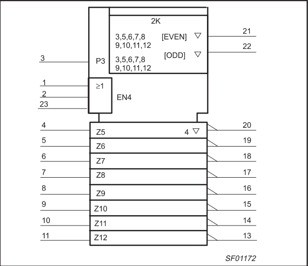
IEEE/IEC SYMBOL – 74F655A
