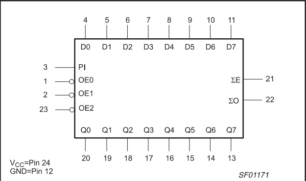
LOGIC SYMBOL (IEEE/IEC) – 74F656A
