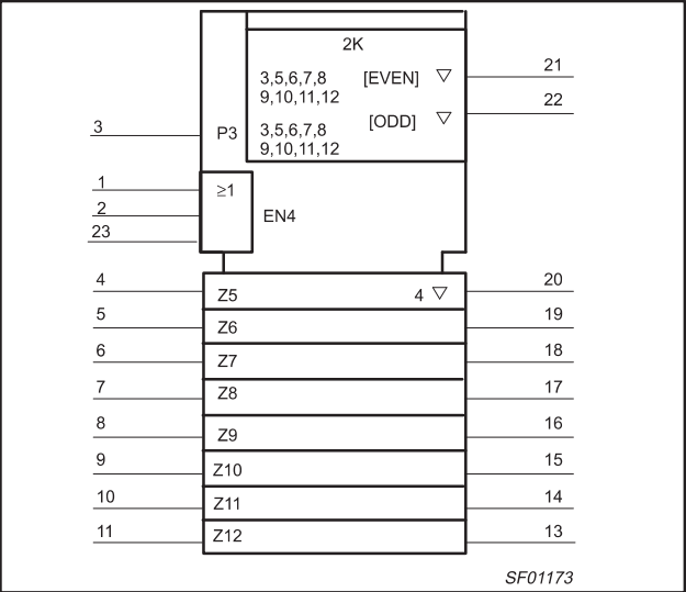
LOGIC SYMBOL (IEEE/IEC) – 74F656A
