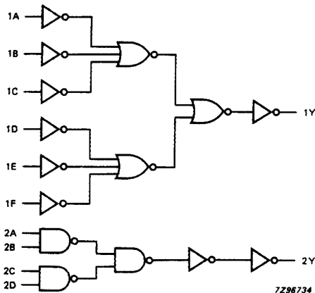
Fig.5 Logic diagram.
