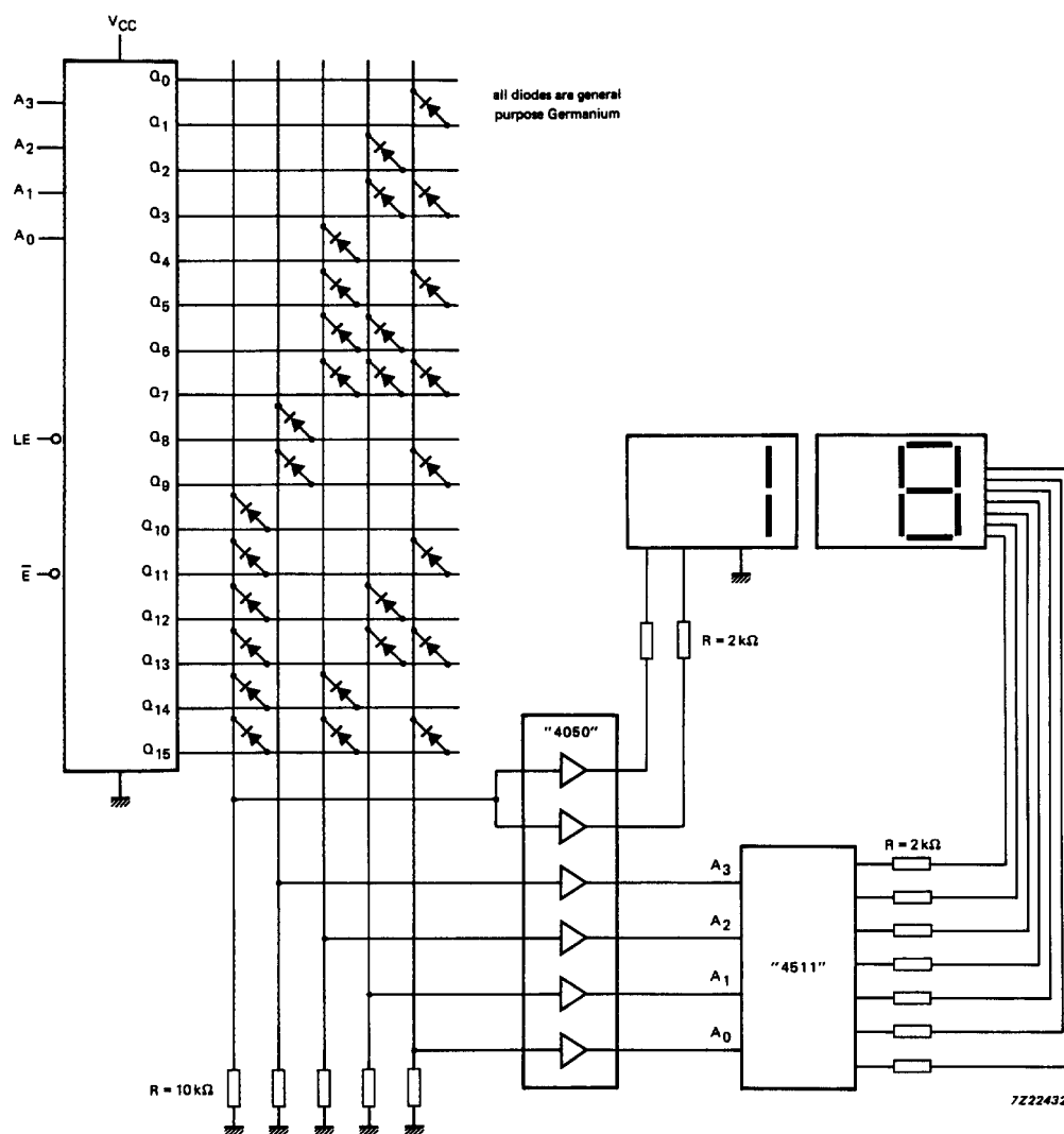
Fig.8 Code-to-code conversion; hexadecimal to BCD.
