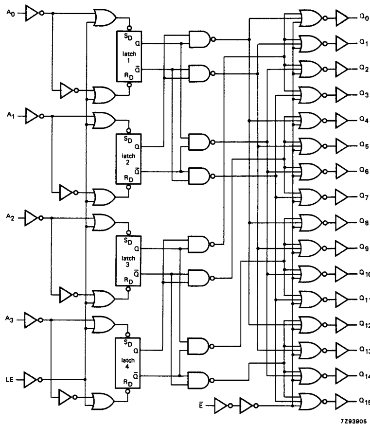
Fig.5 Logic diagram.
