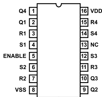
CD4043BMS TOP VIEW
