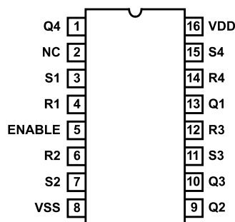
CD4044BMS TOP VIEW
