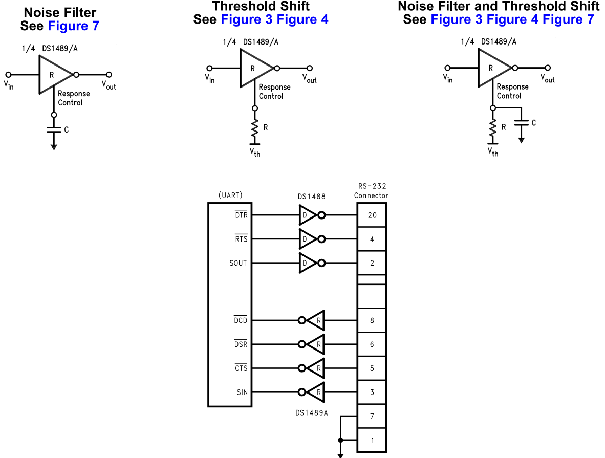
Figure 9. Application of DS1488, DS1489A and UART
