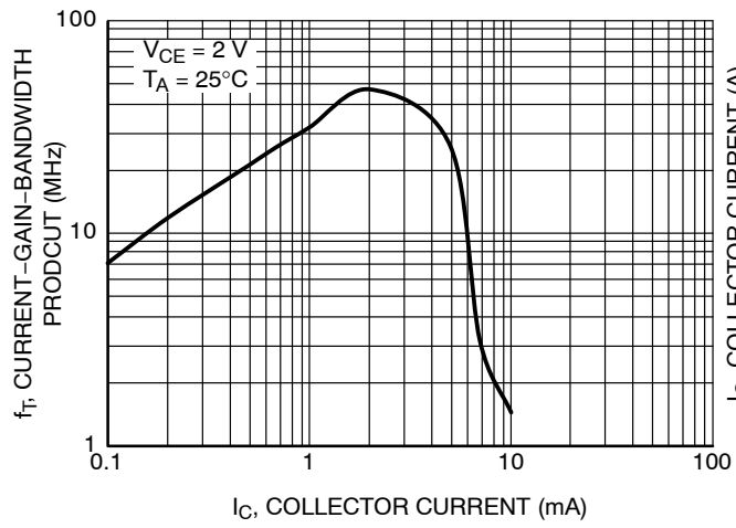
Figure 4. Current-Gain-Bandwidth Product
