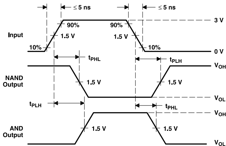
VOLTAGE WAVEFORMS
