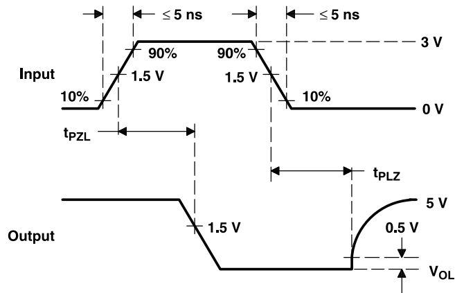
VOLTAGE WAVEFORMS
