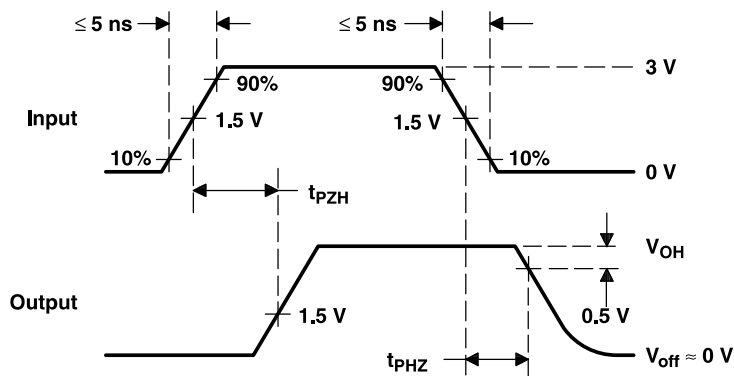
VOLTAGE WAVEFORMS
