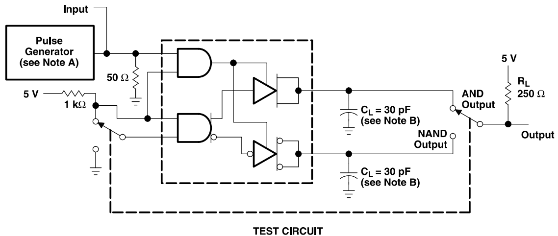
TEST CIRCUIT
